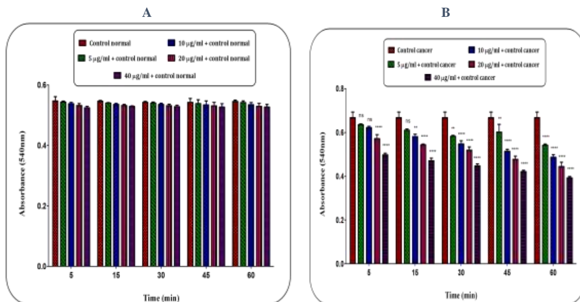
Figure 4. Mitochondrial swelling assay. The effect of E.schistosa (5, 10, 20 and 40 µg/ml) venom on mitochondrial swelling in the liver mitochondria isolated from the normal (a) and cancer (b) groups. Data are showed as mean ± SD (n=3). ** and **** show a significant difference in comparison with the corresponding control (P<0.01 and P<0.0001, respectively).
