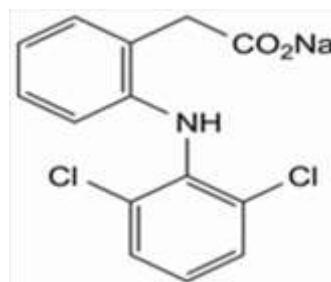
Figure 1. Chemical Structure of Diclofenac sodium.
