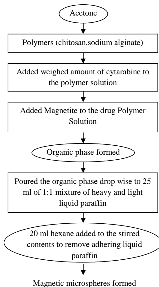
Figure 1. Method of formulation of magnetic microspheres by continuous solvent evaporation method.
