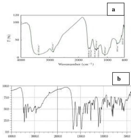
Figure 2. FTIR Spectrum of a)chitosan, b)cytarabine.
