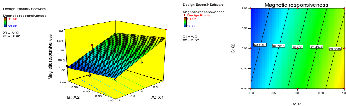
Figure 6. Response surface graph for magnetic responsiveness.
